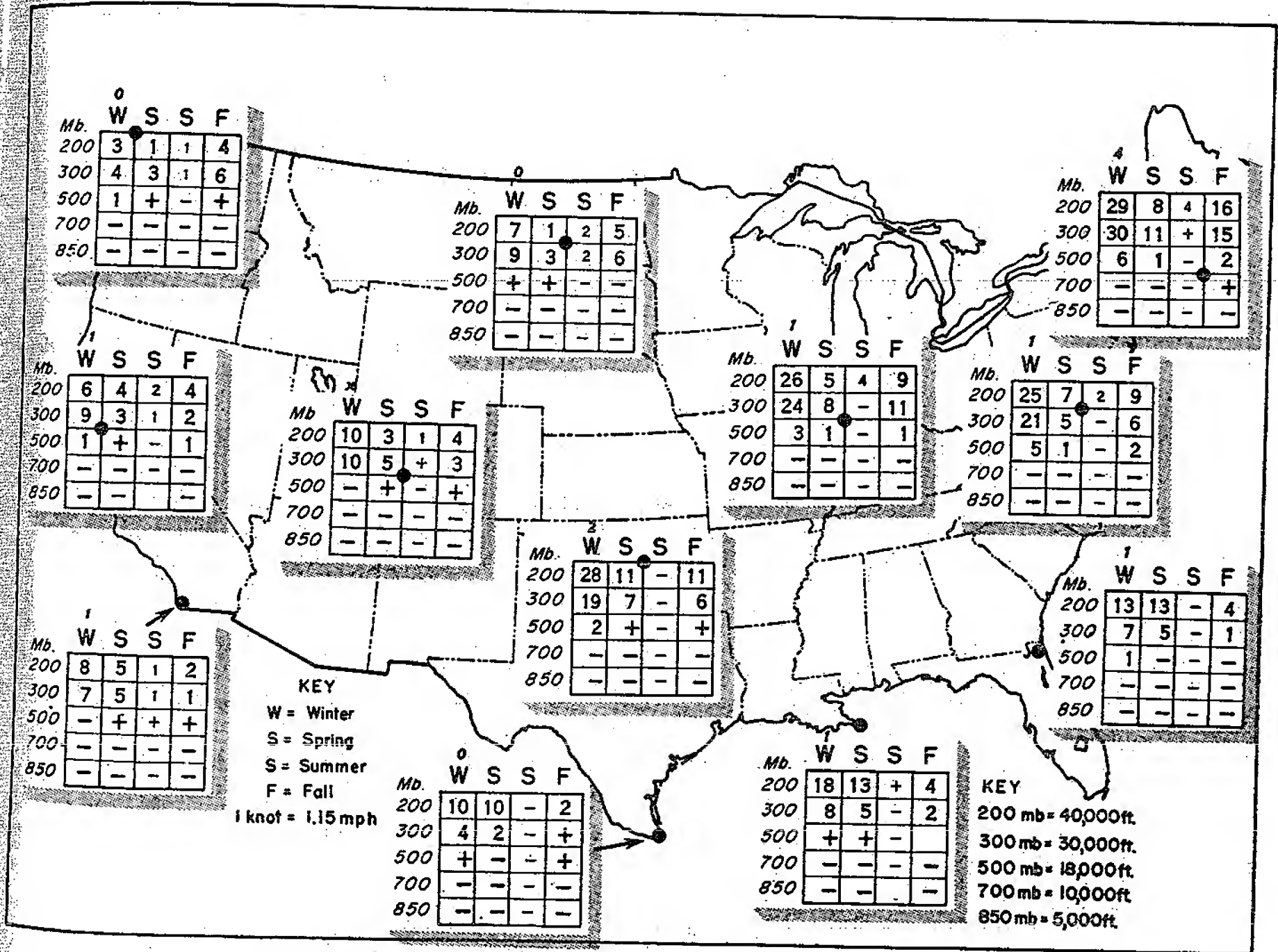
Figure 9. Percentage frequency of winds over 100 knots (115 mph).
